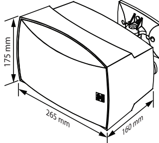
SIDE VIEW FORMAT 20
