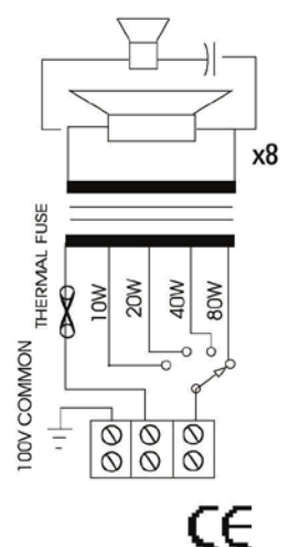
circuit diagram MCS80T/EN
