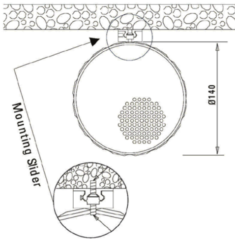
front view unit: mm
